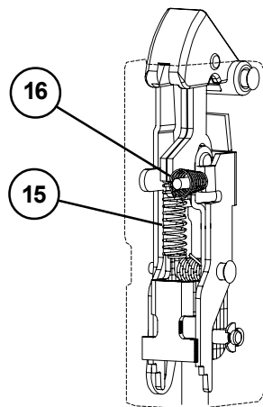
7847 Top Latch
