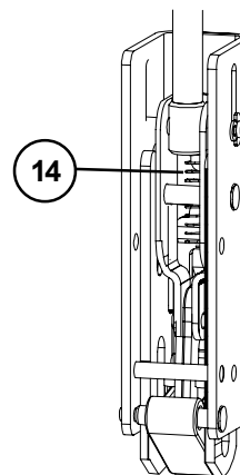
7847 Bottom Latch
