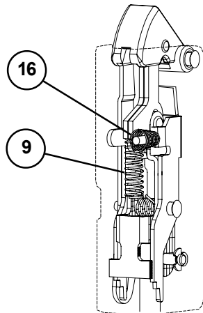
7847 Top Latch
