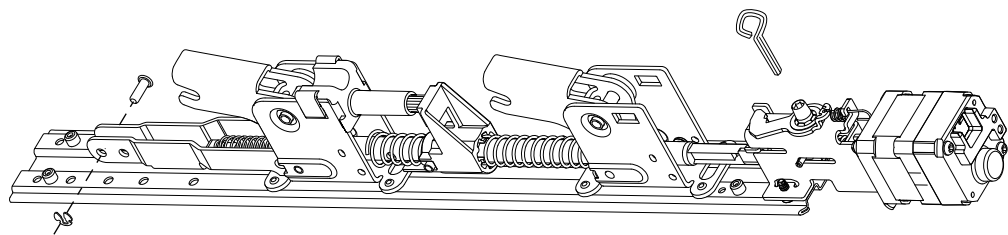
QELA Baseplate with Dogging (replaces EL-HD Baseplate)
